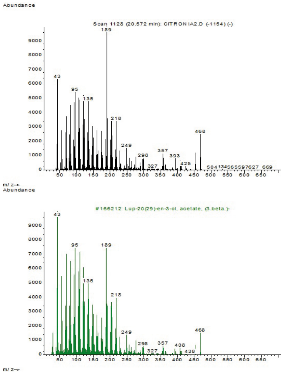
Fig. S11. Mass spectrum of compound at RT = 20.572 min and its similar mass spectrum pattern with Lup-20 (29)-en-3-ol, acetate (NIST library).
