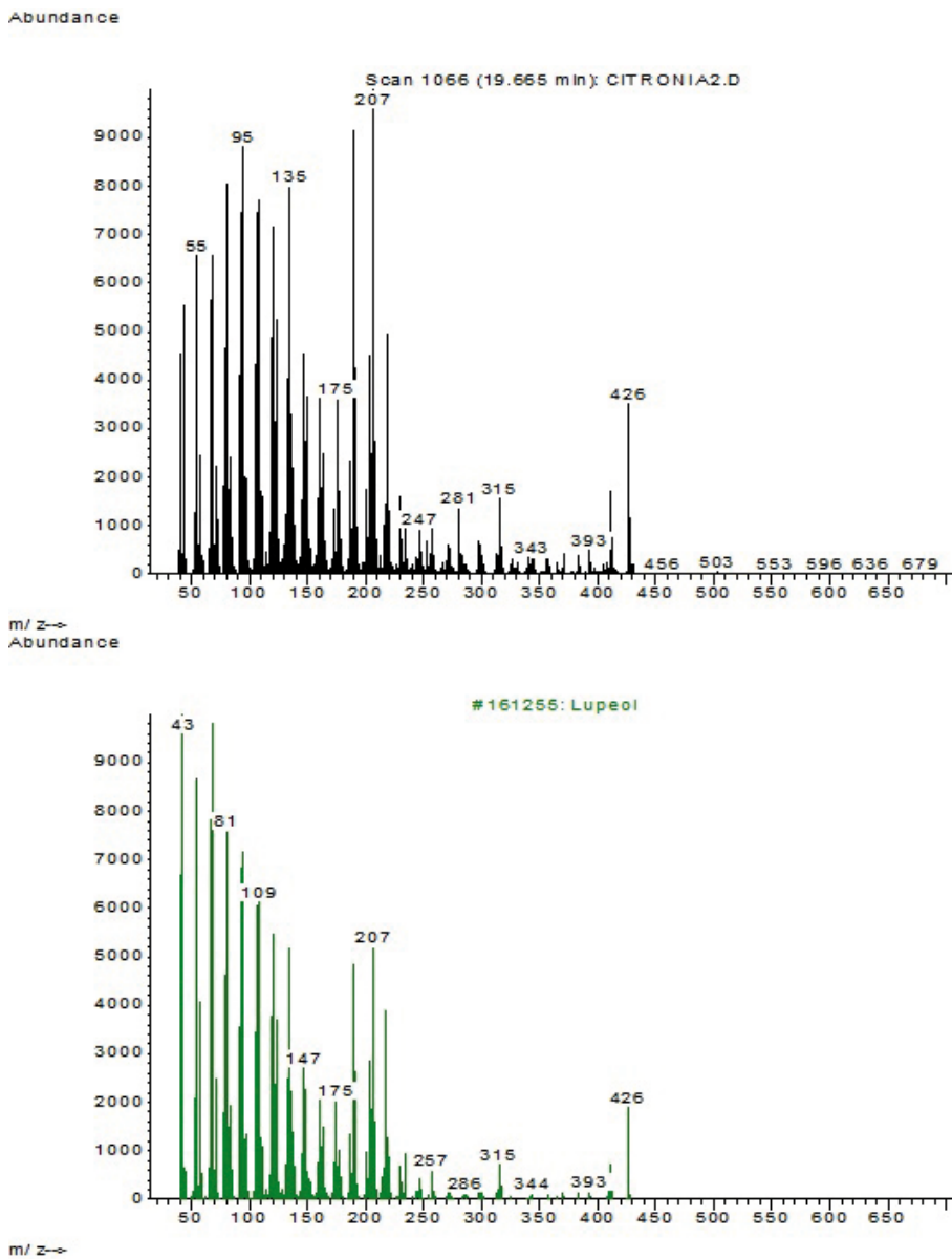
Fig. S10. Mass spectrum of compound at RT = 19.665 min and its similar mass spectrum pattern with Lupeol (NIST library).
