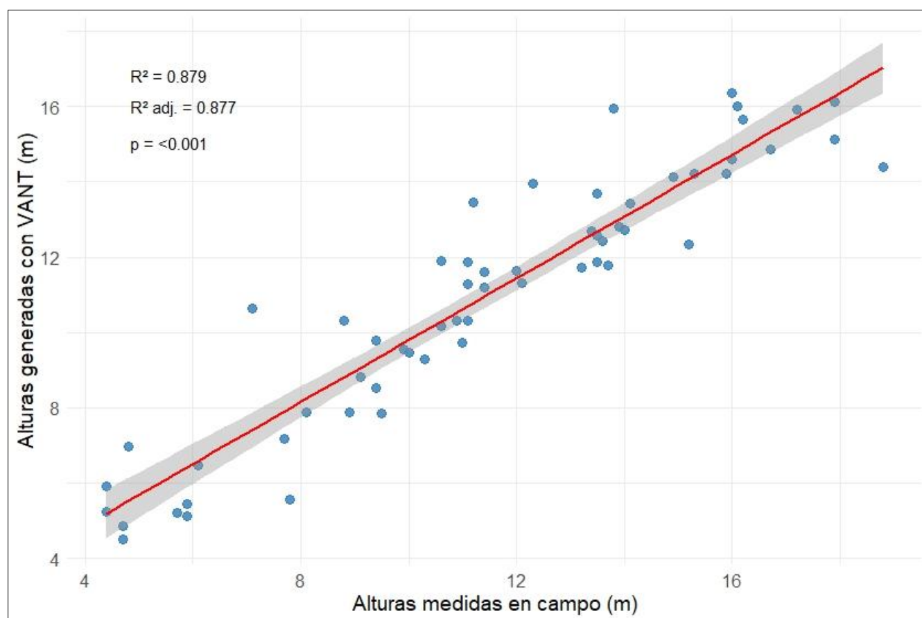
Figura 4. Relación de alturas estimadas con VANT vs alturas medidas en campo. Figure 4. Relationship of heights estimated with UAV vs heights measured in the field.
